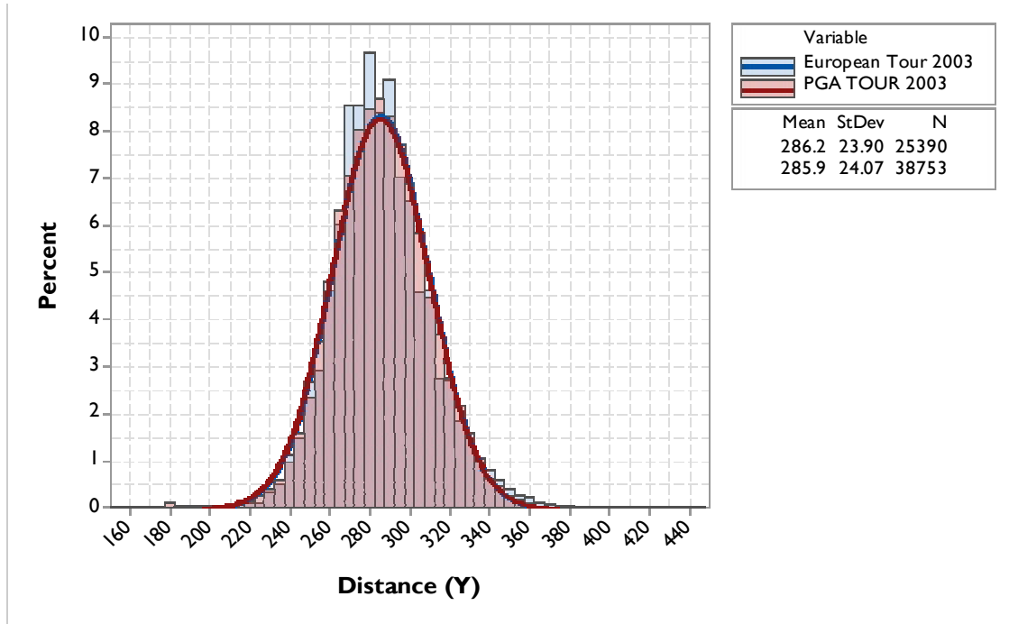
Figure 8. The distribution of distances on “measured” driving holes on the European and PGA TOUR in 2003.
