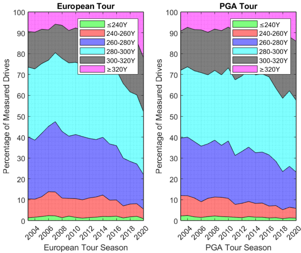
Figure 10. The distribution of drives on “measured” driving holes on the European and PGA tours 2003-2020.
