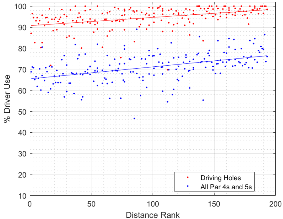
Figure 11. Percentage Driver usage vs distance rank on the PGA TOUR in 2020.
