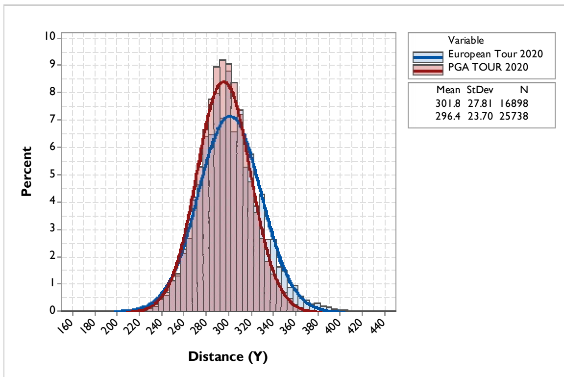
Figure 9. The distribution of distances on “measured” driving holes on the European Tour and PGA TOUR in 2020.
